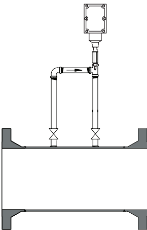
Insertable OOD™ on a main pipe, with 2" MNPT seal housing
