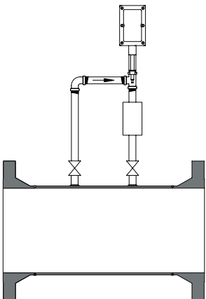
Insertable OID™ on a main pipe, with 2" MNPT seal housing
